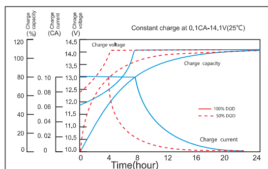
Charging characteristic
